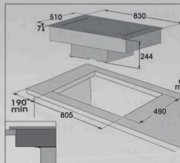
IN APPOGGIO - SURFACE MOUNTED
