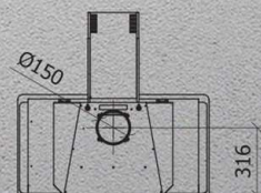
VISTA POSTERIORE BACK VIEW
