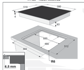
A FILO - FLUSH MOUNTED
